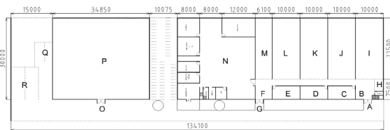
Gambar 1. Layout Awal Gudang PT. MKM
