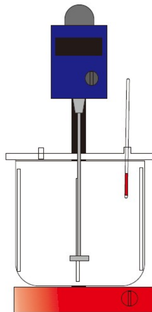
Gambar 4. Alat Maserator
